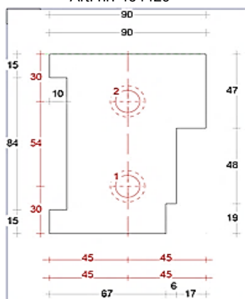
Neut links 90mm Sponning Bu 67mm Art. nr. 464430
